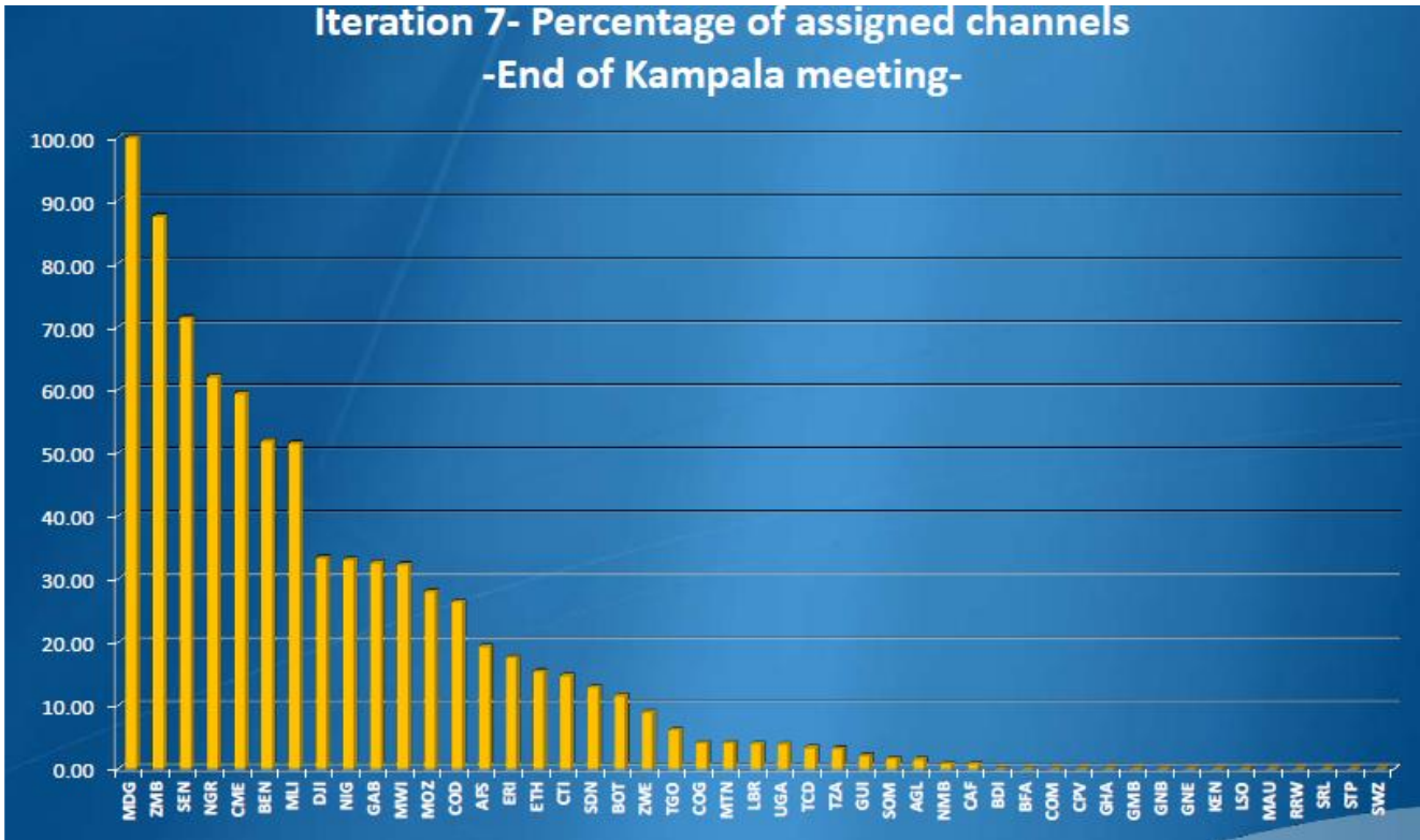
Figure 2: Iteration 7 - Attainability percentage to achieve 4 DTT multiplexes or more within the band 470–694 MHz band
