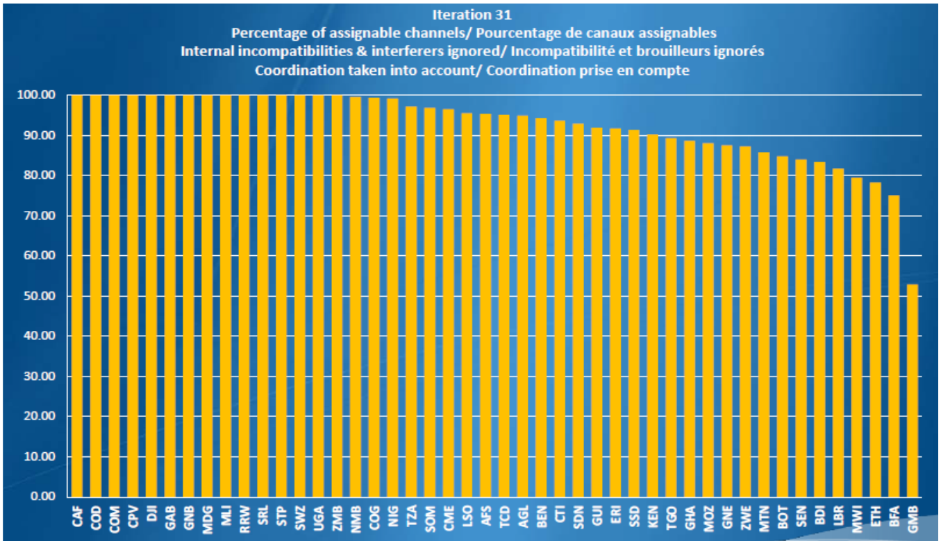
Figure 4: Iteration 31 - Attainability percentage to achieve 4 DTT multiplexes or more within the band 470–694 MHz band
