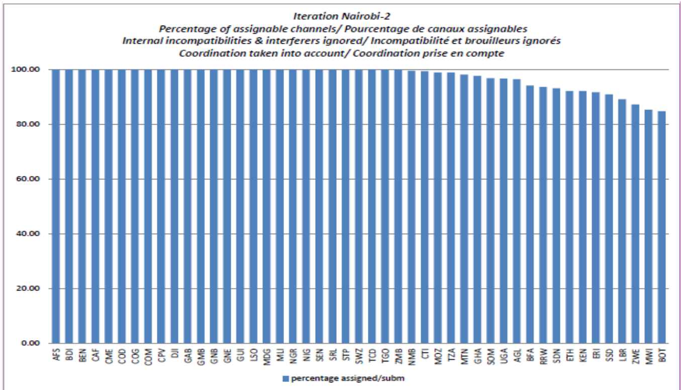
Figure 5: Iteration Final - Attainability percentage to achieve 4 DTT multiplexes or more within the band 470–694 MHz band
