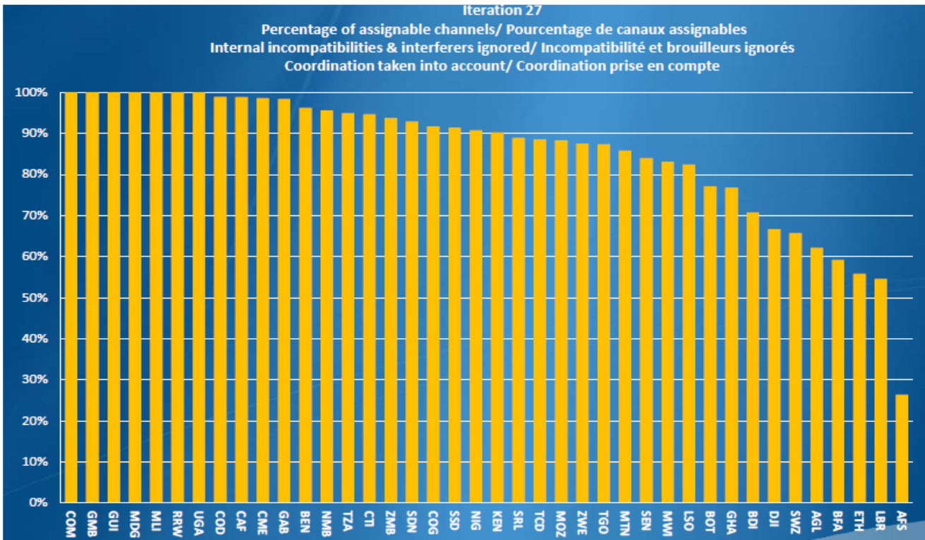
Figure 3: Iteration 27 - Attainability percentage to achieve 4 DTT multiplexes or more within the band 470–694 MHz band
